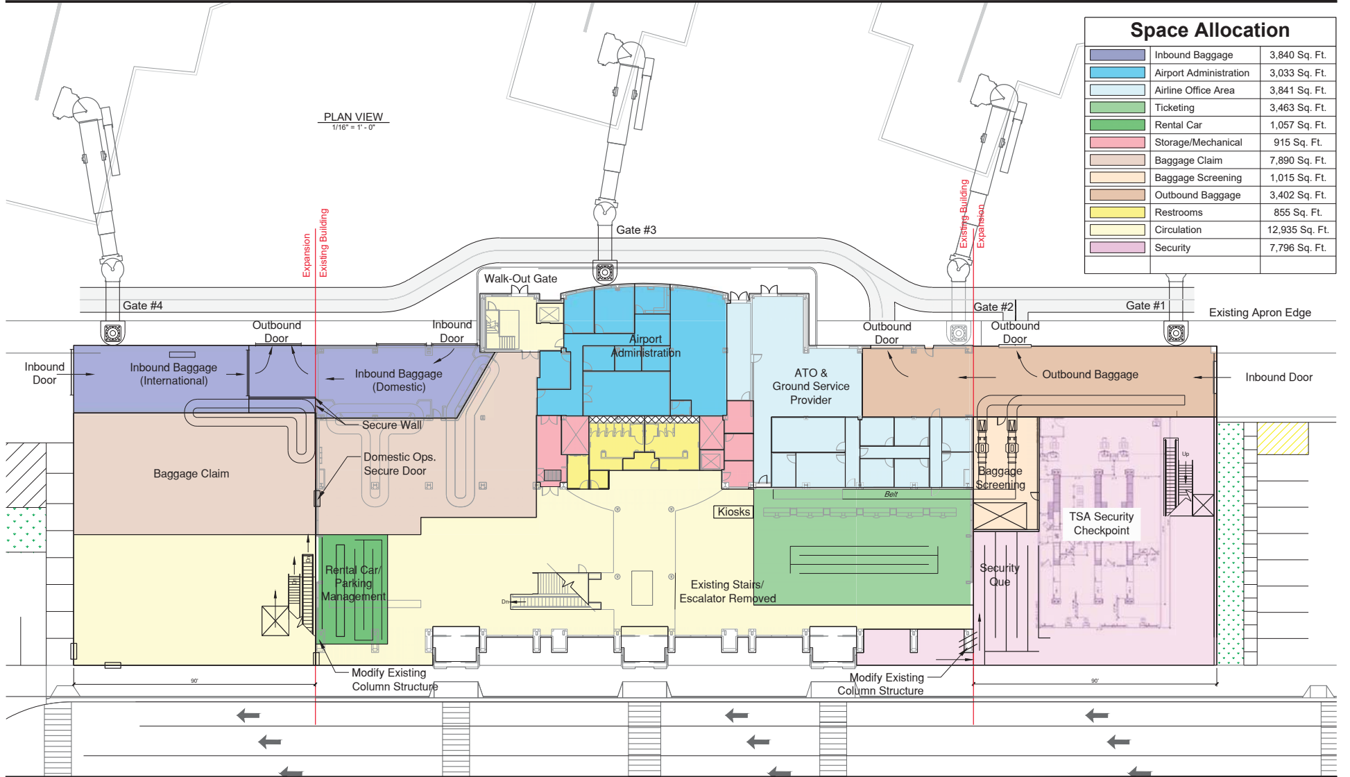
First Floor Plan Concept
