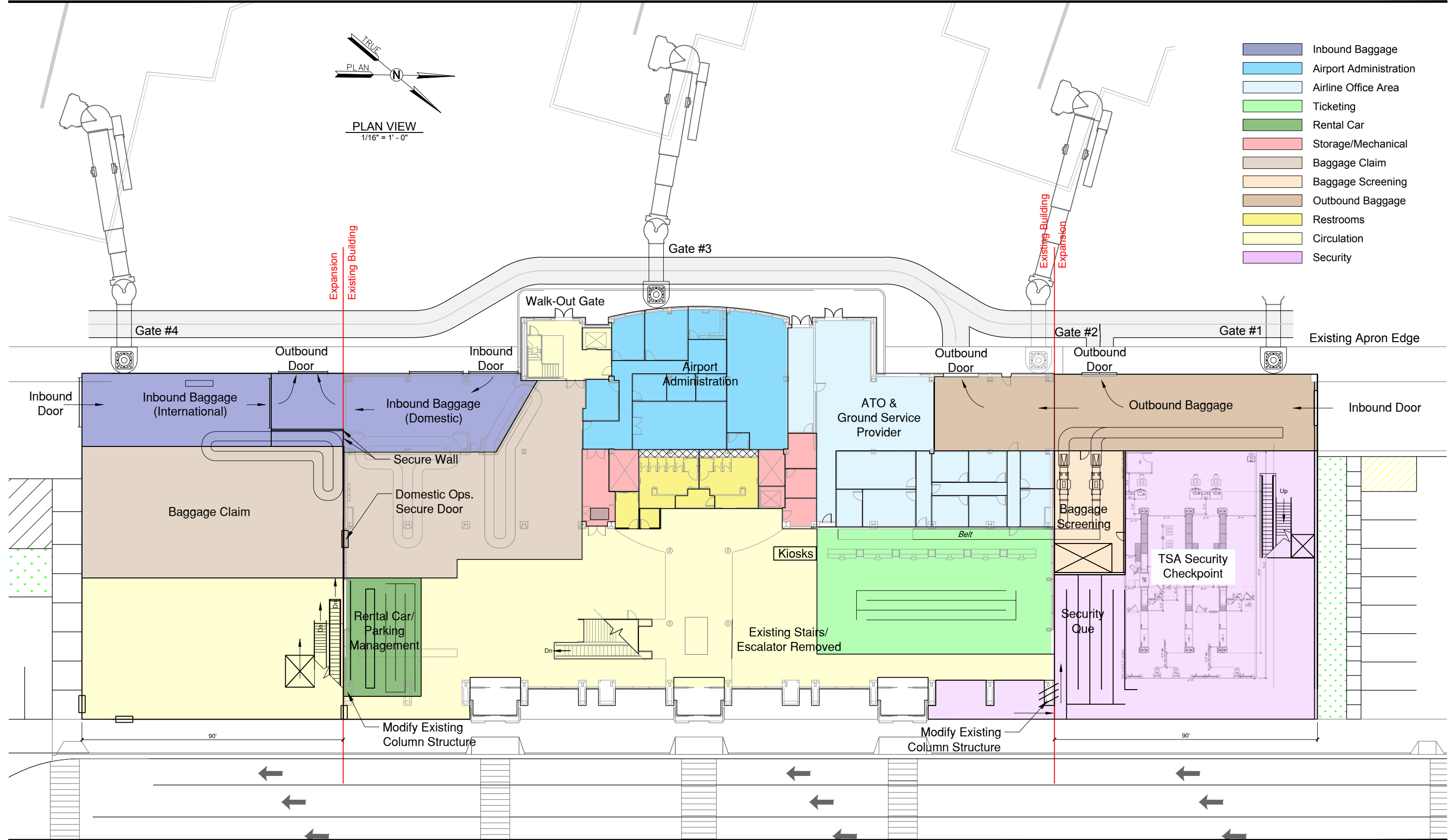
First Floor Plan Concept
